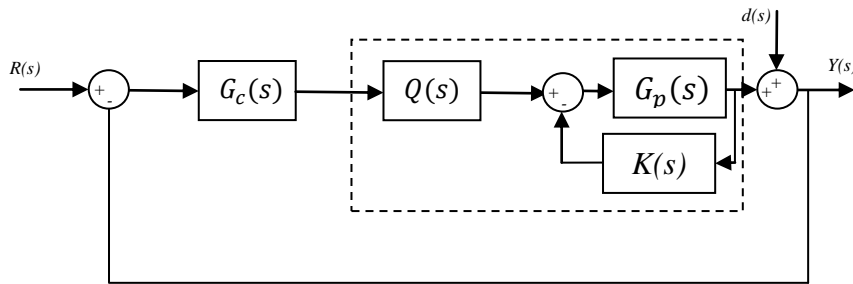
Figure (3.14): Modified IMC for Unstable systems
