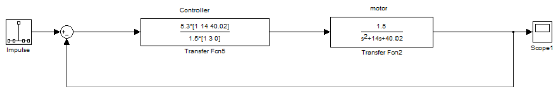
Figure (3.5): Overall closed Loop system
